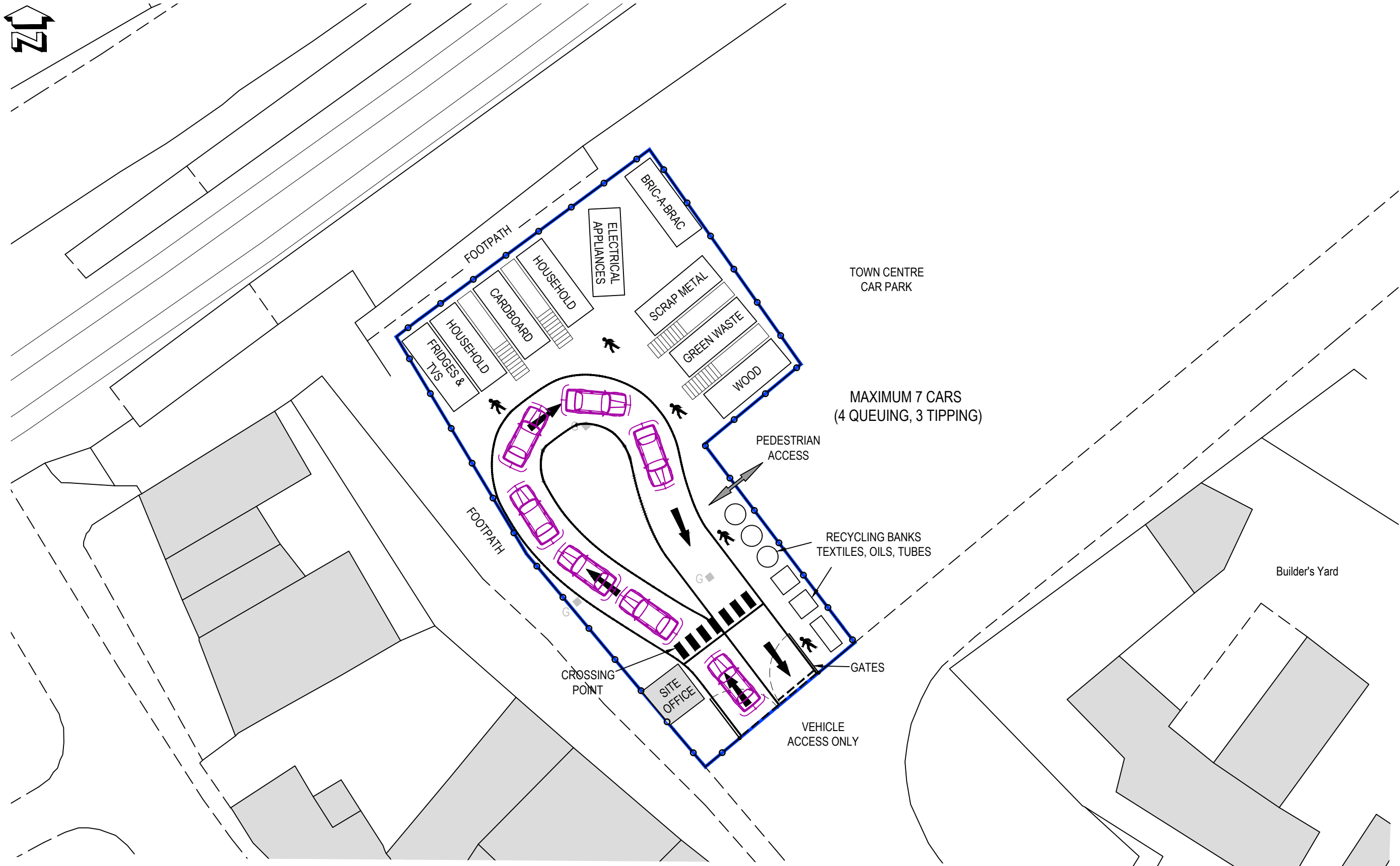
SITE LAYOUT
